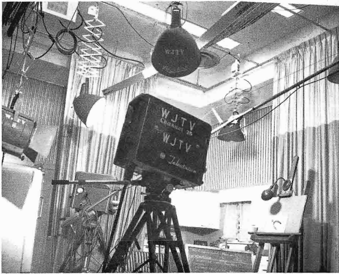
FIG. 5. View of a corner of the WJTV studio which shows a typical lighting and camera arrangement.
