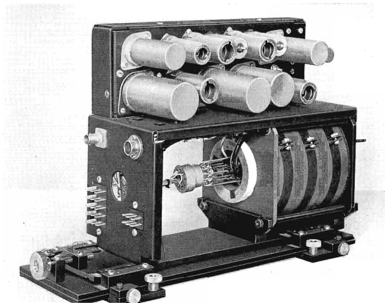
FIG. 4. Single vidicon chassis showing focus, centering and alignment mechanisms.
