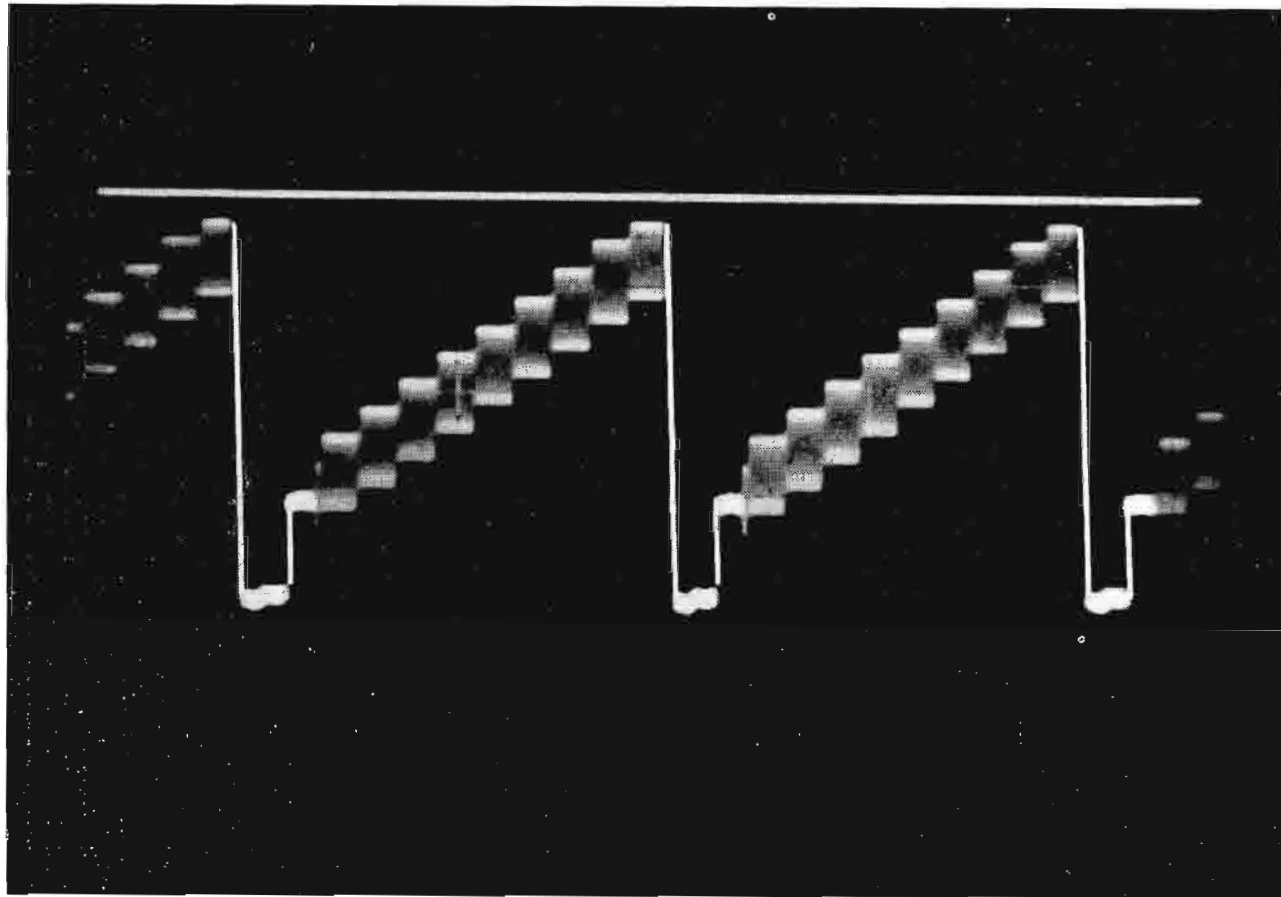
FIG. 10. TTU-12A output step-wave, channel 59, 11.3 KW output.
