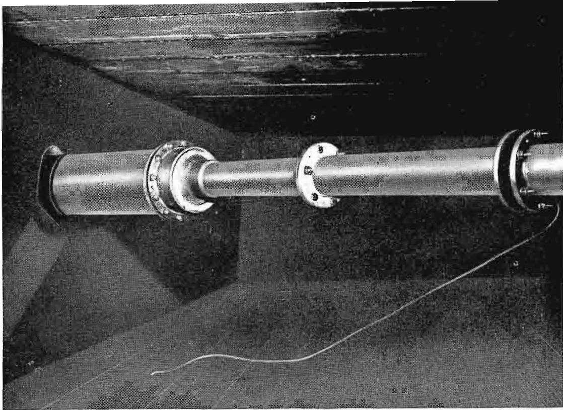
FIG. 5. This photo and the one for Fig. 6 was taken in the "loft" above the transmitter room. It shows the 3 1/8" UHF transmission line from the Filterplexer merging with a 6 1/8" line leading to the tower. The 3 1/8" 50 ohm line is efficiently matched to the 6 1/8" 75 ohm line by a reducer transformer (MI-19387-4). The 1/4" copper tubing coming through floor delivers dry-nitrogen to pressurize line to the antenna.
