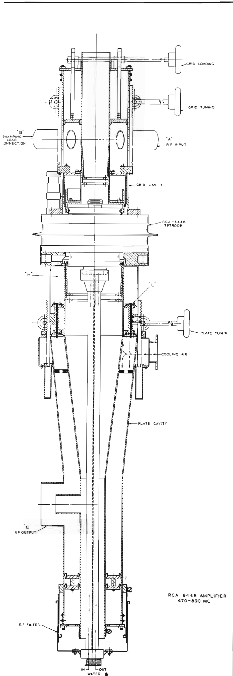
FIG. 3. Cross-sectional view of the 6448 tube and cavity. Note the rugged, simplified mechanical arrangement which results in simplified tuning—and easy handling because of the small overall cavity size.
