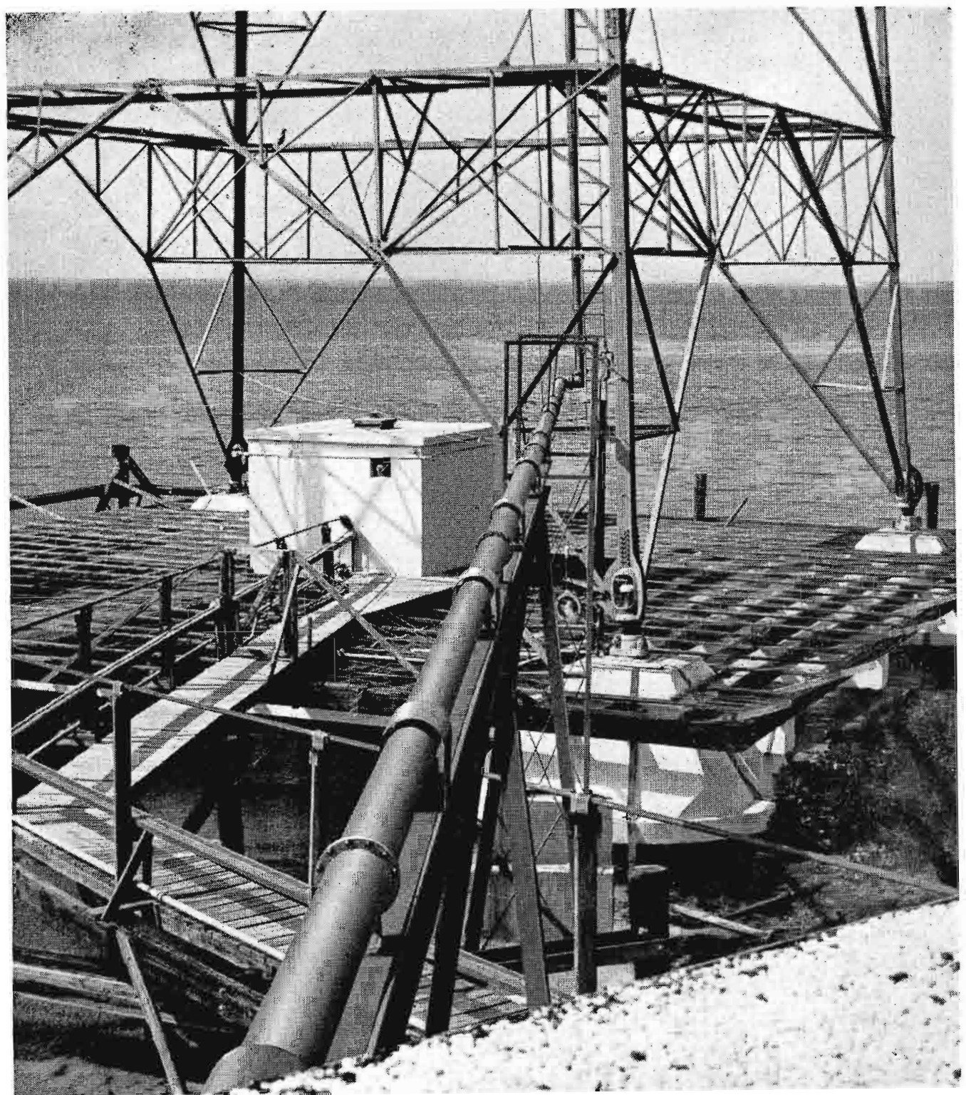
FIG. 7. View showing 6 1/8" transmission line leaving transmitter building and method of supporting horizontal run to the tower.
