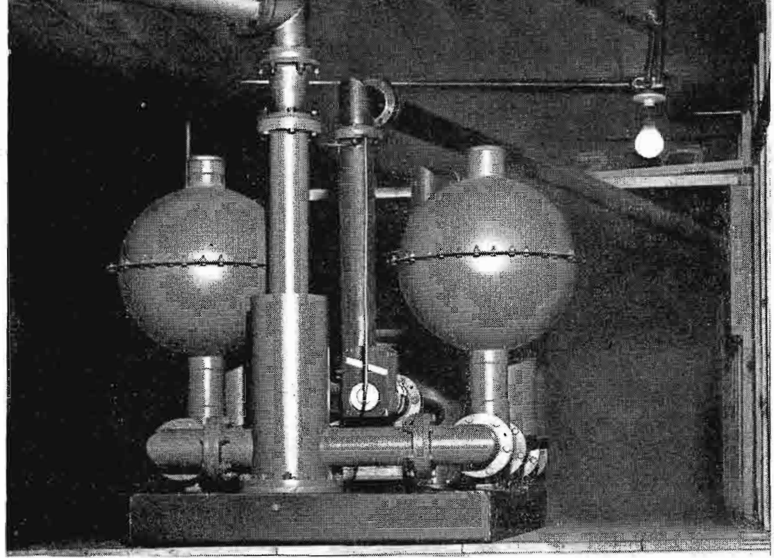
FIG. 6. The Filterplexer is located in a section of the loft above the transmitter. This permits a saving of space on the transmitter room floor and still provides facility for maintenance and insertion of an RF load and watt meter for transmitter checks. The line at upper left proceeds to the 6 1/8" reducer transformer in the adjacent photo.
