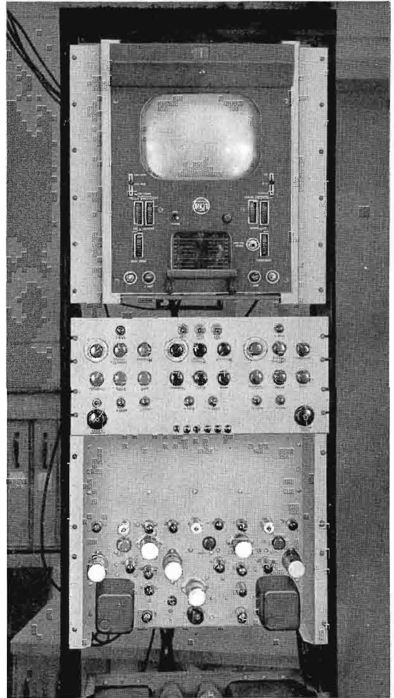
FIG. 11. The Processing Amplifier (bottom) and Operating Control Panel (center) are shown rack mounted beneath an RCA TM-6B Master Monitor. These units comprise the control function of the 3-Vidicon Color Camera Chain.
