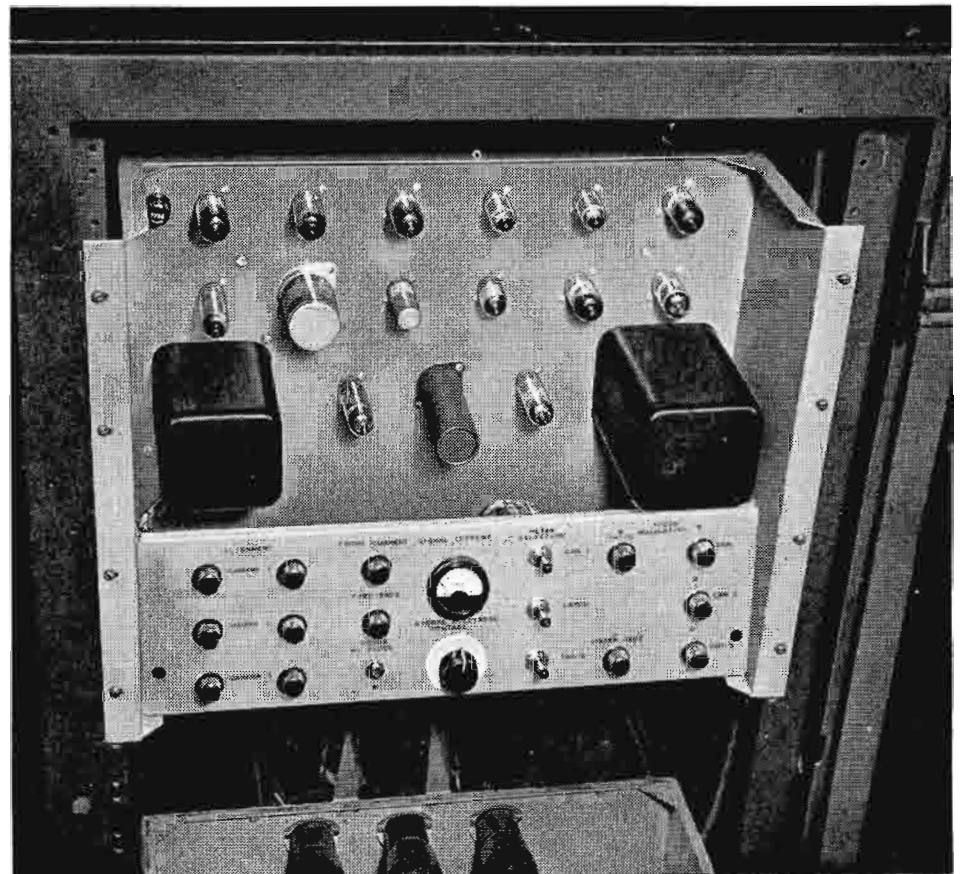
FIG. 10. Auxiliary Control Unit.
