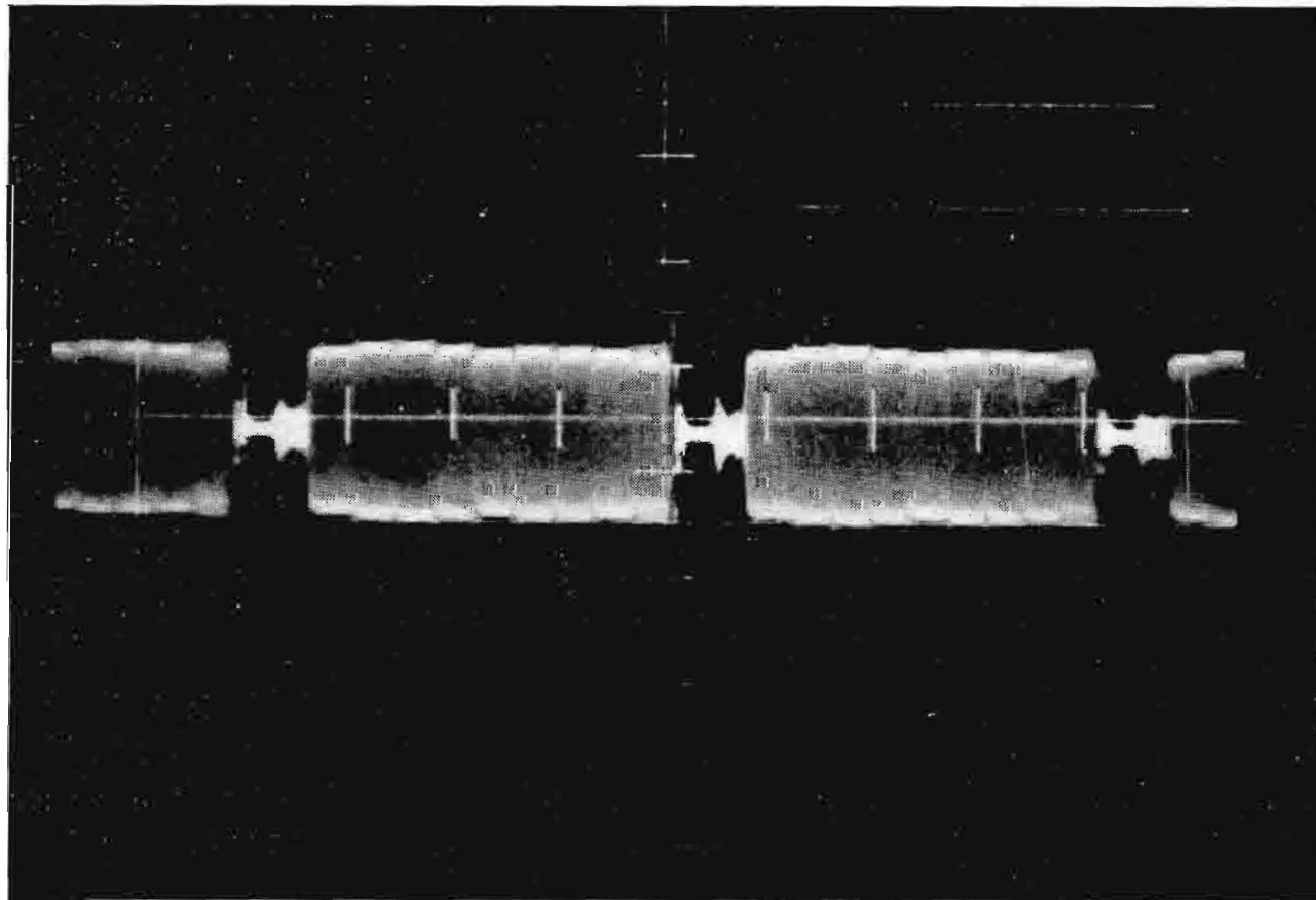
FIG. 11. TTU-12A output, color sub-carrier incremental gain, channel 59, 11.3 KW output.
