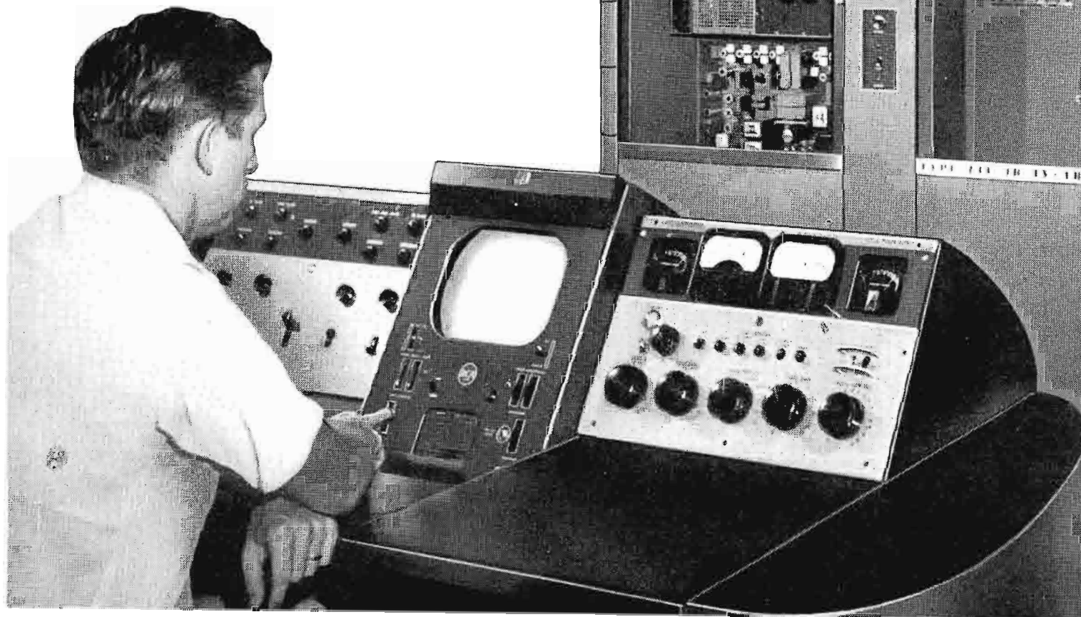
FIG. 4. View of RCA 1 KW UHF Transmitter with RCA TTC-1B Transmitter Control Console in foreground. The TTC-1B provides centralized control of transmitter, visual and aural program circuits.
