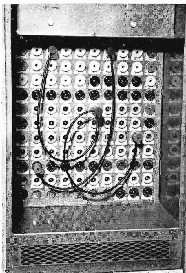
FIG. 15. Close-up of the Davis Switchboard Panel which contains 65 color-coded load circuits—each connected to a "pigtail" attached to lighting grid.
