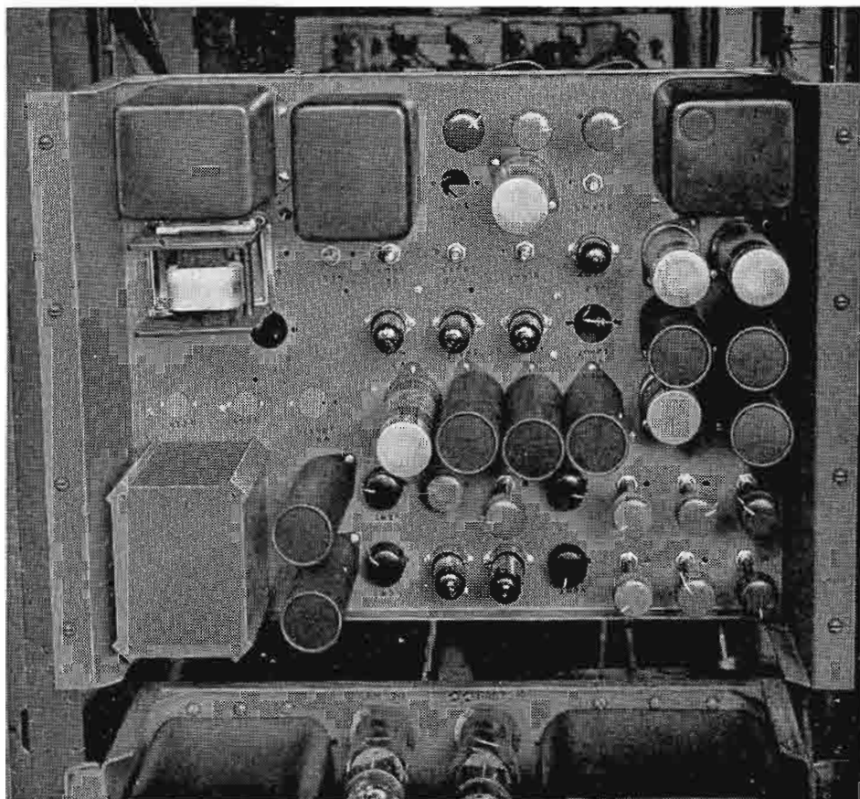
FIG. 9. Deflection Assembly.
