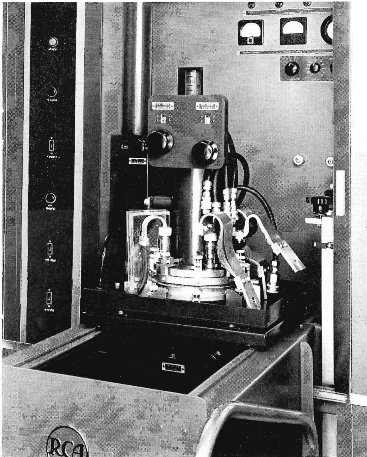
FIG. 5. A spare "P.A." cavity, supplied as a part of the transmitter, simply glides from a dolly into proper position in the P.A. cabinet. Compactness of the tetrode and unique cavity construction permits the operator, unassisted, to replace the complete final stage with an auxiliary amplifier within five minutes.
