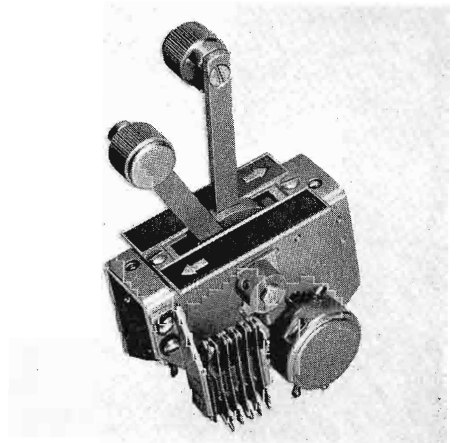
FIG. 8. The fader mechanism located in the control panel of the TS-5A.
