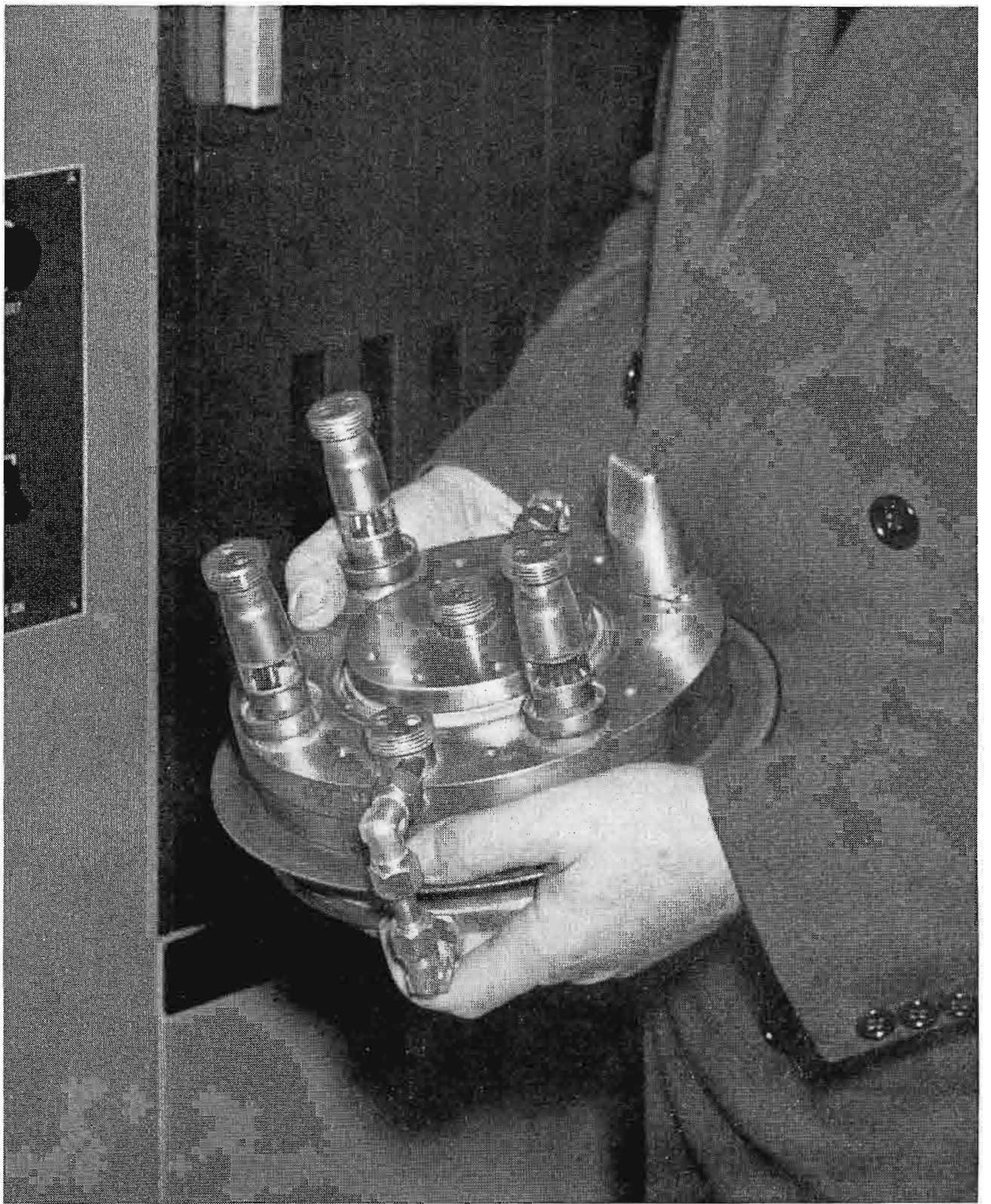
FIG. 4. Closeup view of the new small-size, RCA 6448 used in the TTU-12A Transmitter. The same conventional tube (RCA Type 6448) is used in the Aural and Visual "P.A." Use of conventional types of tubes throughout results in economical operation, easy maintenance, and simple, straightforward circuitry.
