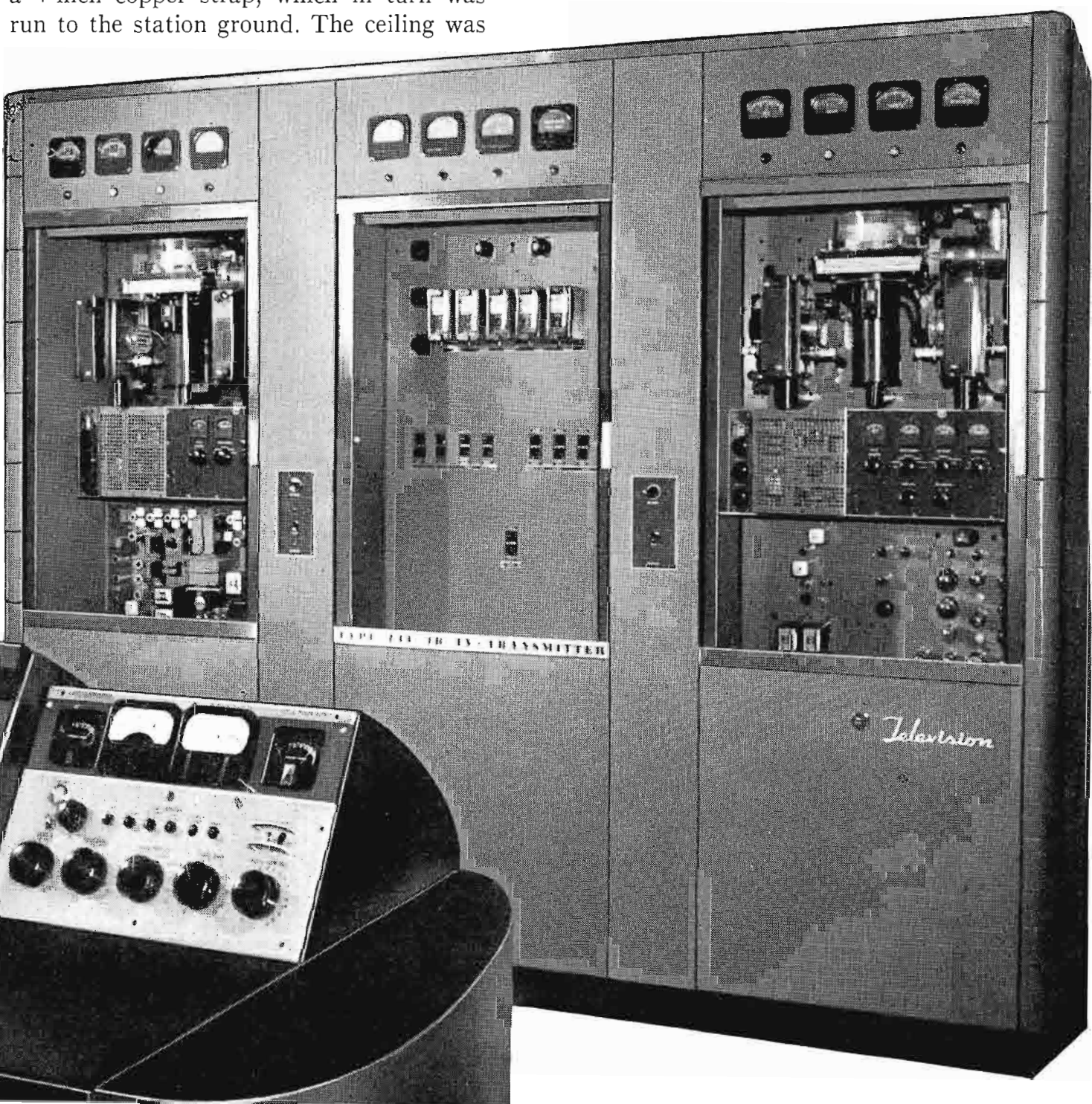
FIG. 4. View of RCA 1 KW UHF Transmitter with RCA TTC-1B Transmitter Control Console in foreground. The TTC-1B provides centralized control of transmitter, visual and aural program circuits.
