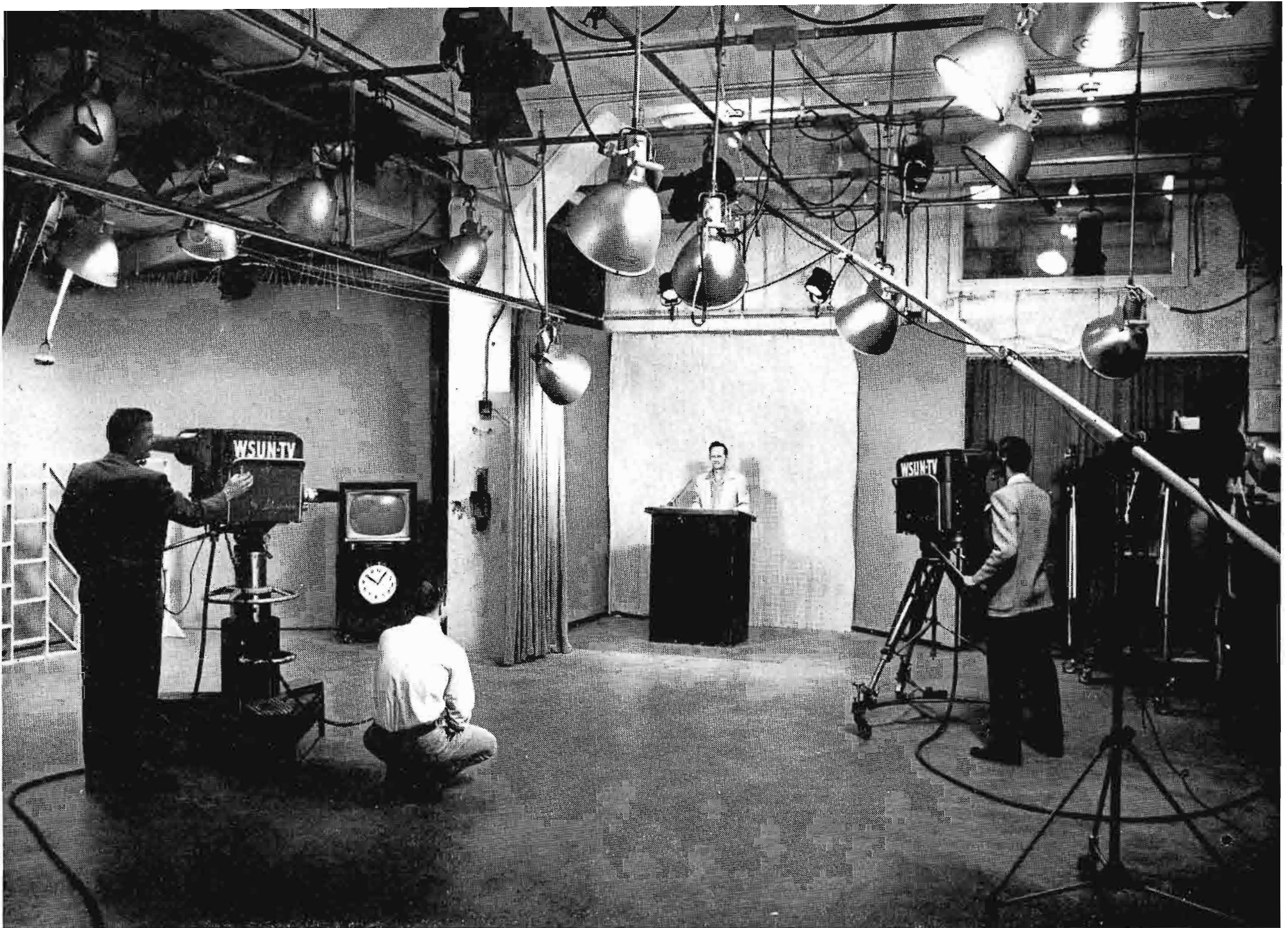
FIG. 13. A studio scene showing clean orderly arrangement of equipment. This is attributed to the convenient lighting system shown in Figs. 14 and 15 and described in the text under "TV Lighting equipment." RCA TK-11A studio cameras are shown—pedestal-mounted on left, tripod-dolly-mounted on right. Century boom holds RCA 77-D microphone.
