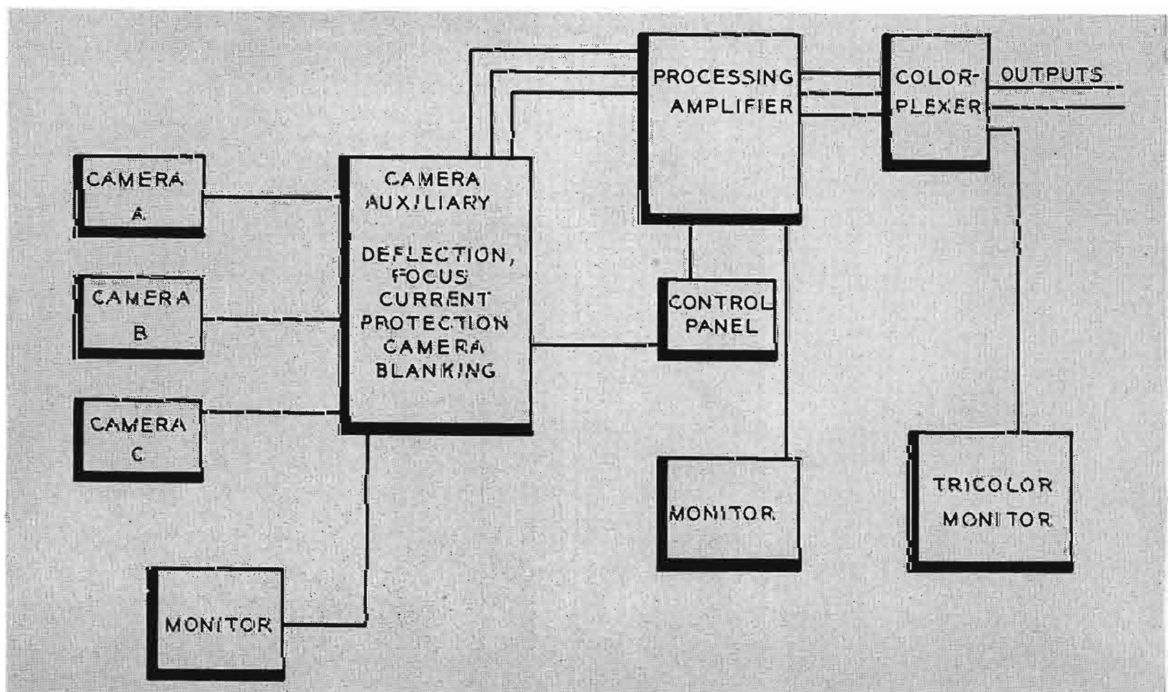
FIG. 15. Block diagram of the 3-Vidicon Color Film System showing general packaging of the various components in the system.
