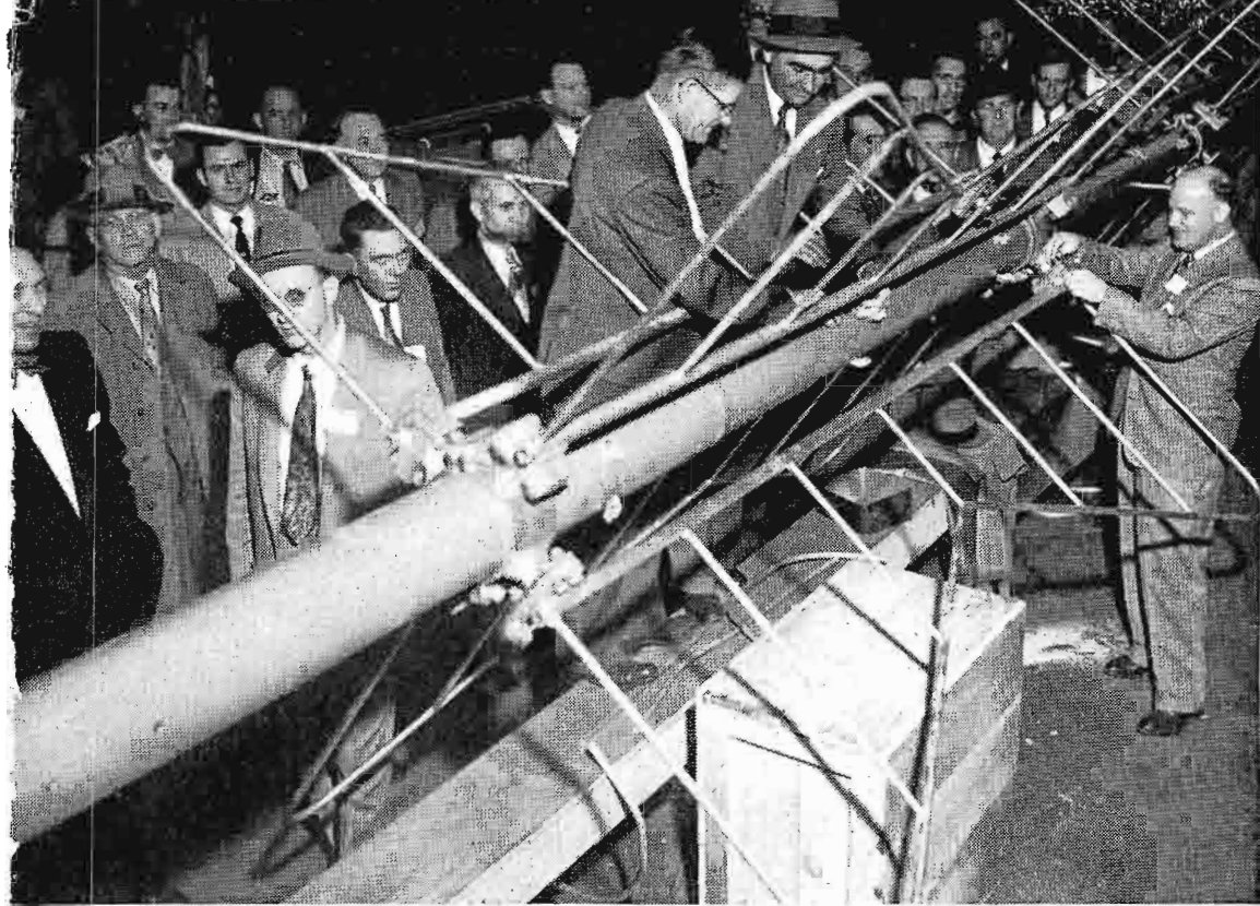
A. H. Super, of RCA, accompanies the Erectors' Forum group during a demonstration of the Superturnstile Antenna.
