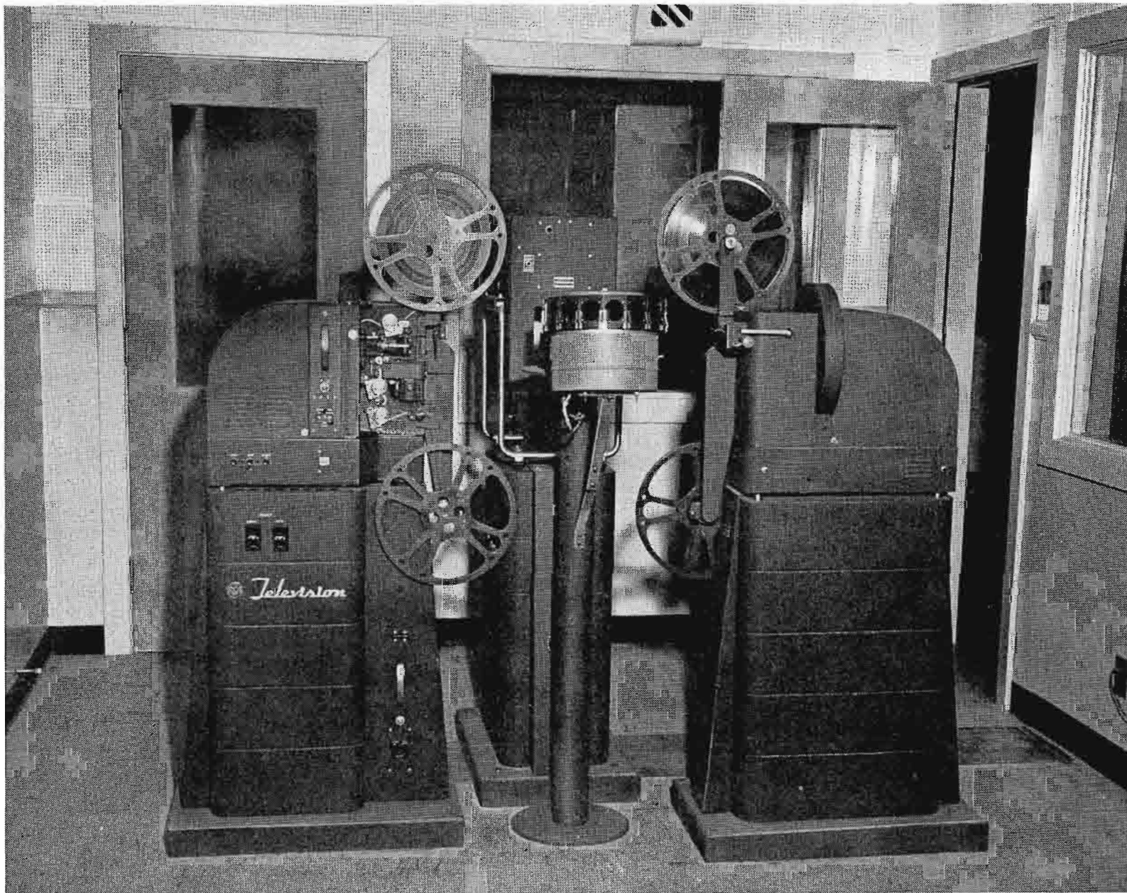
FIG. 7. View of the WJTV film projection room showing the use of RCA 16mm projectors, TK-20 film camera, and automatic slide projector.
