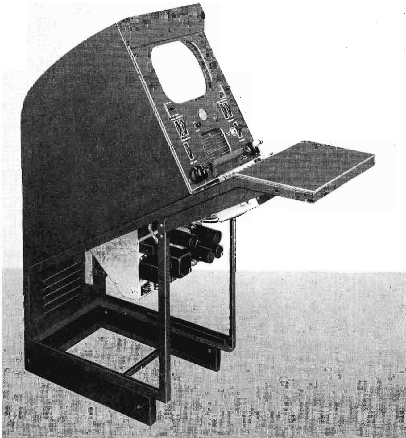
FIG. 7. The TS-5A Switcher is shown below with its control panel and amplifier unit mounted with a TM-6B Master Monitor in a standard console housing. ▼
